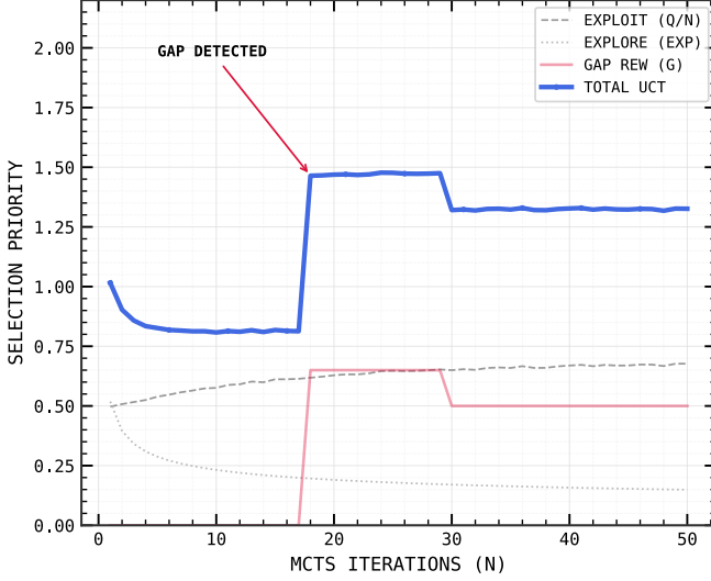
Fig. 2. UCT-Gap Reward Dynamics. This plot illustrates the component values of the modified UCT_{gap} selection metric across 50 simulation iterations. At iteration 17, the framework identifies a high-priority information gap, causing the gap penalty term ( \alpha \cdot \text{GapScore} ) to spike. This dynamically overrides the standard exploration-exploitation balance, forcing the algorithm to aggressively pursue targeted conflict resolution until the gap is resolved and the priority score normalizes.
